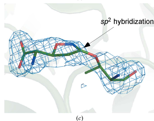
Figure 1 The structure and binding modes of acivicin. (a) The structure of acivicin. Previously reported acivicin-binding configurations in (b) E. coli GGT at 1.65 Å resolution (Wada et al. , 2008) and (c) H. pylori GGT at 1.70 Å (Williams et al. , 2009). An OMIT F_o - F_c map for the acivicin adduct contoured at 2.0\sigma (blue) is overlaid on its stick model of each GGT and bound acivicin.
